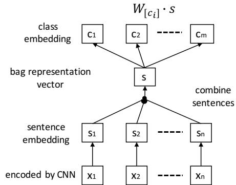
Figure 1: The main architecture of our model.
